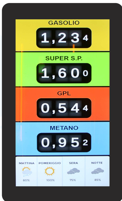
Meteo
